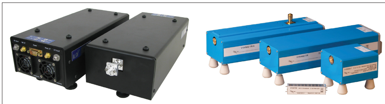
VDI and OML mmWave Modules
